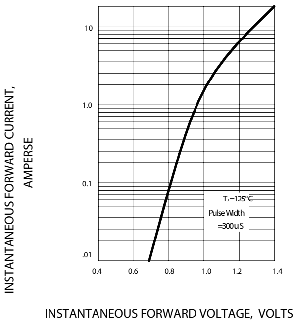
FIG.3 – TYPICAL FORWARD CHARACTERISTIC
